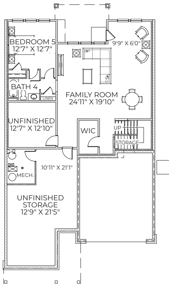
OPTIONAL BASEMENT - STAGE 2
