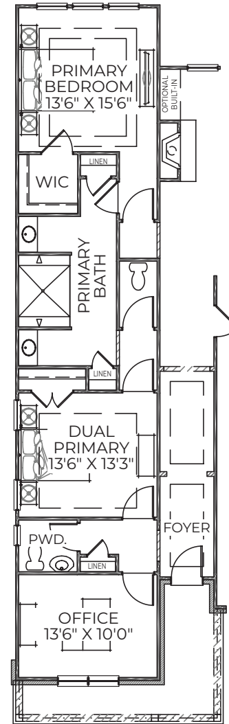
OPTIONAL DUAL PRIMARY #1
