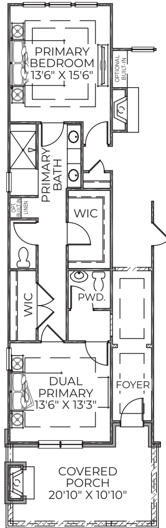
OPTIONAL DUAL PRIMARY W/EXPANDED PORCH
