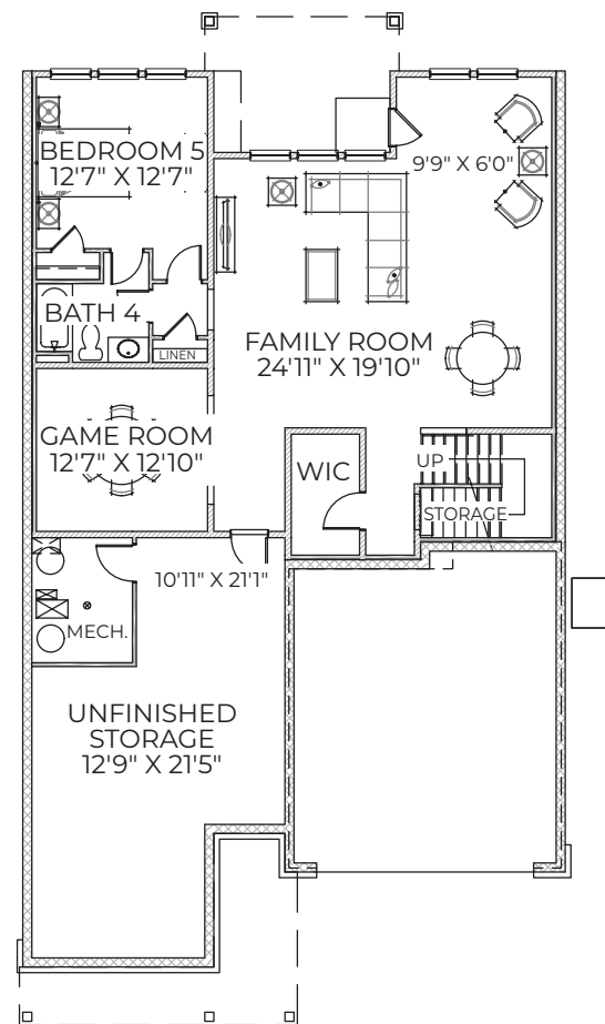
OPTIONAL BASEMENT - STAGE 3
